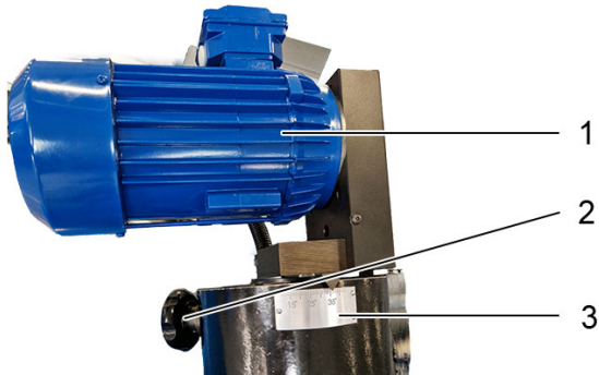
Image 2. Grinder
