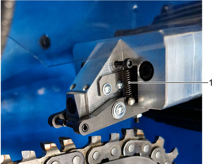
Image 34. Microswitch on sensor arm
