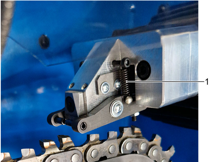
Image 40. Microswitch on sensor arm
