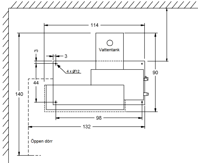
Image 1. Space requirement for machine
