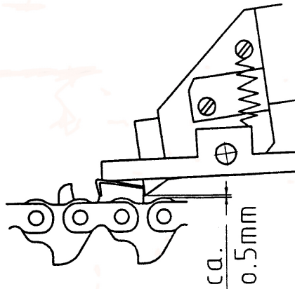
Image 12. Adjusting distance
