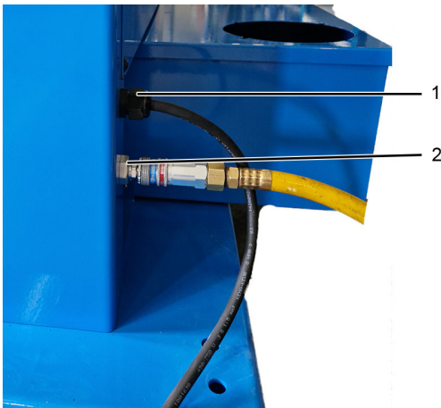
Image 47. Connections
